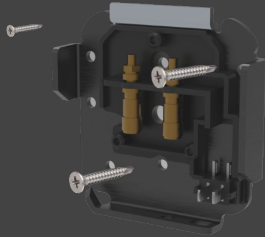
1. MOUNT THE WALL PLATE
